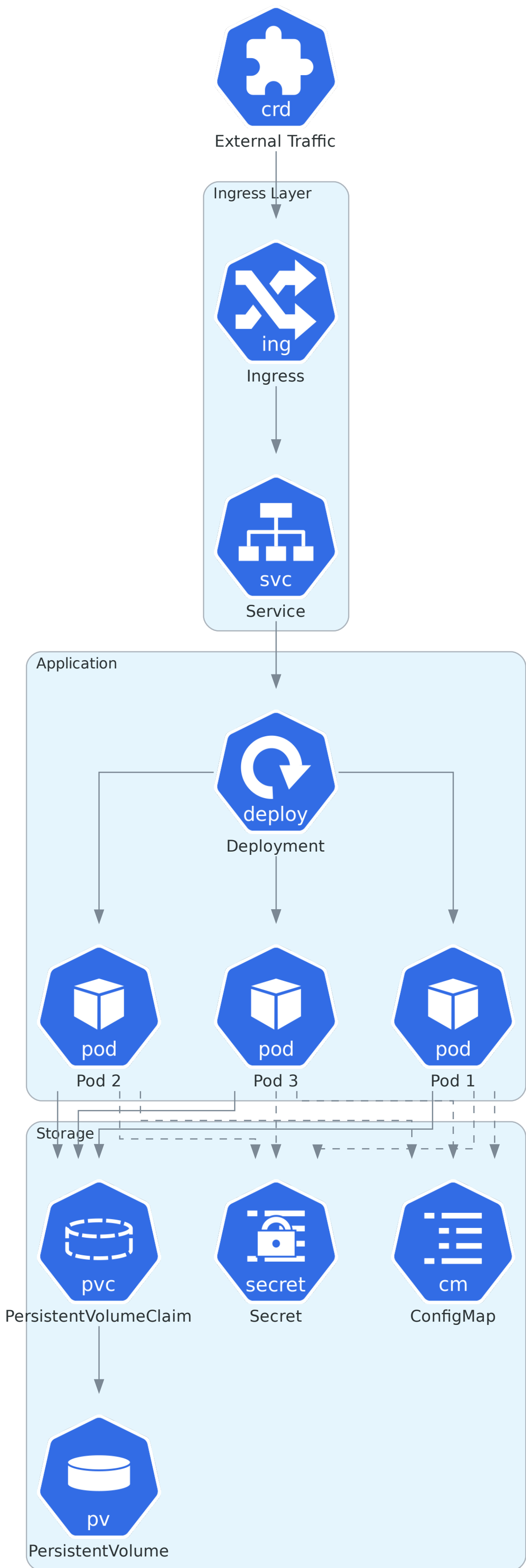
Kubernetes Deployment
